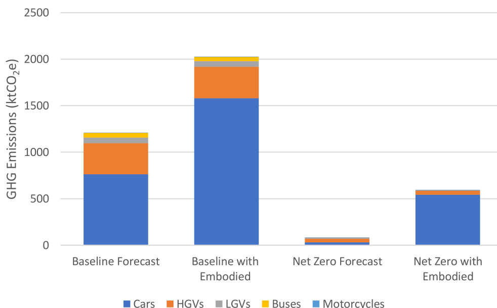
Figure 3.8: The GHG Emissions release in 2050 for the Baseline Forecast and Net Zero Scenario plotted with and without including the embodied emissions of cars that come from battery production, vehicle components and assembly and disposal. Shifting the car fleet to electric vehicles reduces emissions to nearly net zero within Cambridgeshire and Peterborough but emissions are still produced elsewhere as a result.
